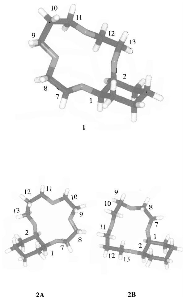
Figure 3. MM^+ calculated geometries for 1, 2A and 2B.
