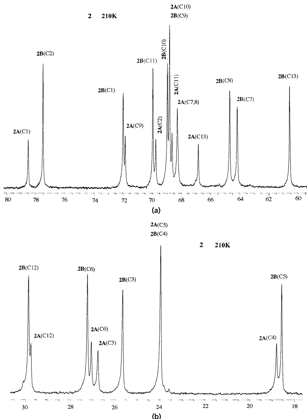
Figure 2. 100 MHz ^{13}\text{C} NMR spectra of 2 (a) oxygenated carbons and (b) non-oxygenated carbons, at 210 K.
