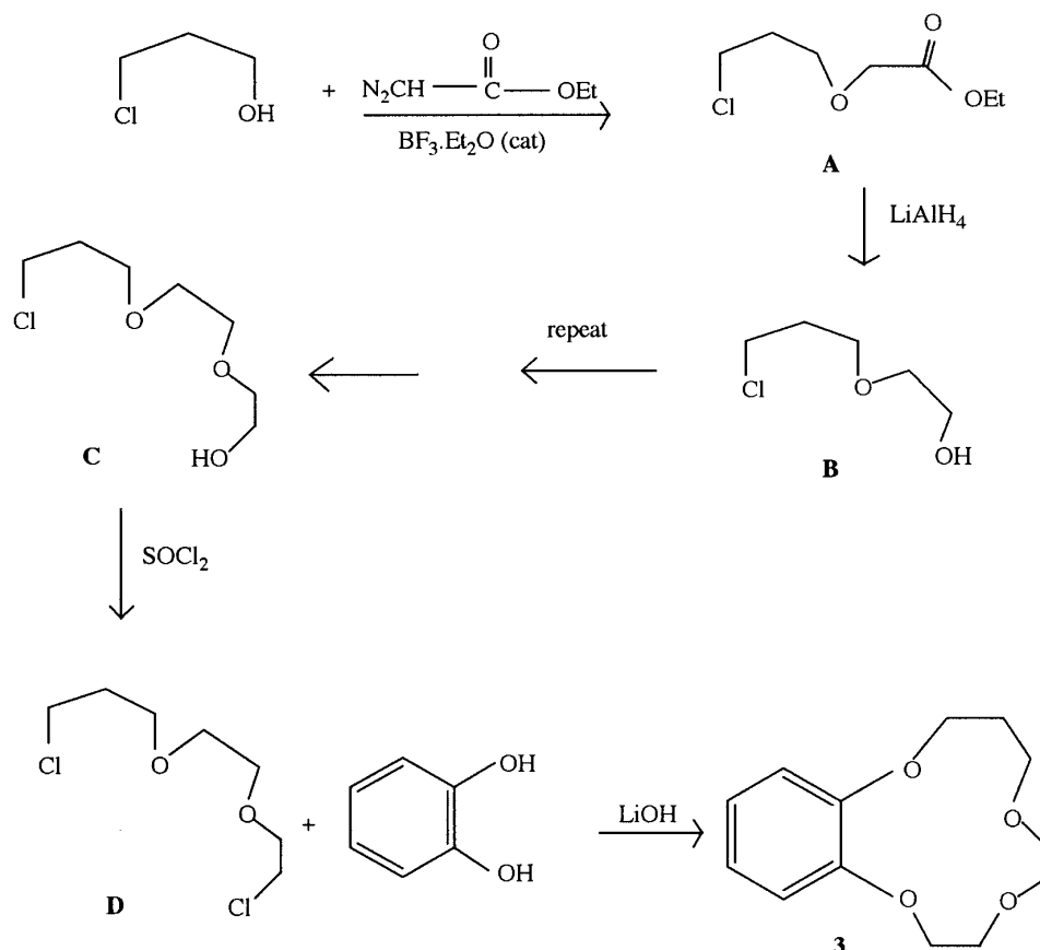
Figure 4. Synthetic scheme for preparation of 3.
