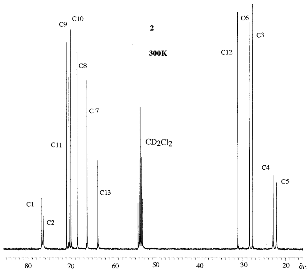
Figure 1. 100 MHz ^{13}\text{C} NMR spectrum of 2 at 300 K.
